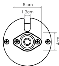
Original Range Wall Bracket
