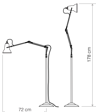
Original 1227™ Floor Lamp
