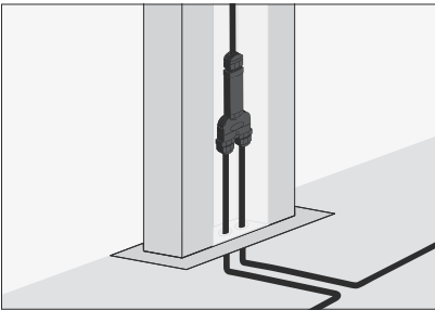
Y-Verbinder: Y-connector:
