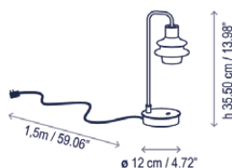
Interruptor Proxy Dimmer / Proxy Dimmer Switch
